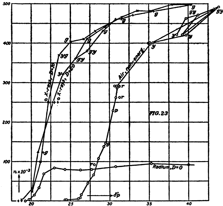
FIG. 23.—Efficient nucleations ( n ) in dust-free air, energized or not, as specified at different exhaustions ( \delta p ). Table 14.
